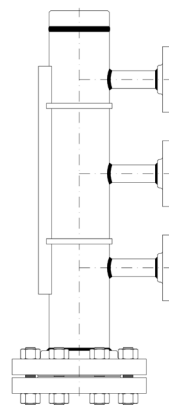
Option 1 with 3 process connections (consult factory)
